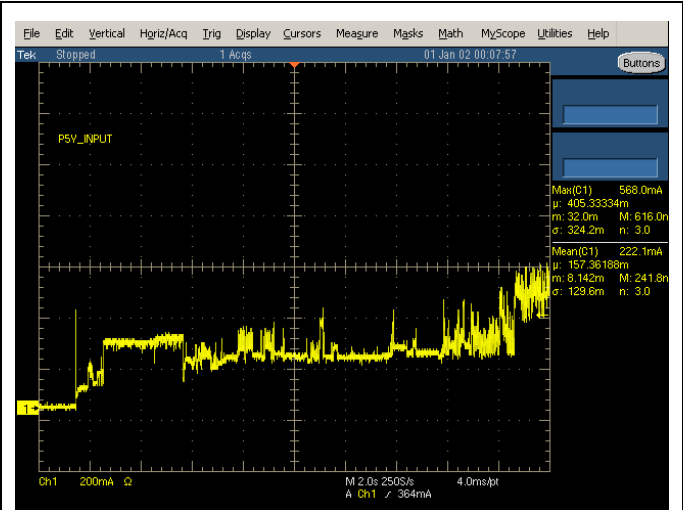
Fig. 2: P5V_INPUT (AC:110V)
