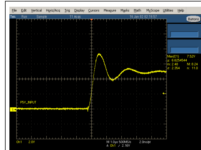
Fig. 3: P5V_INPUT (Zoom in) (AC:110V)
