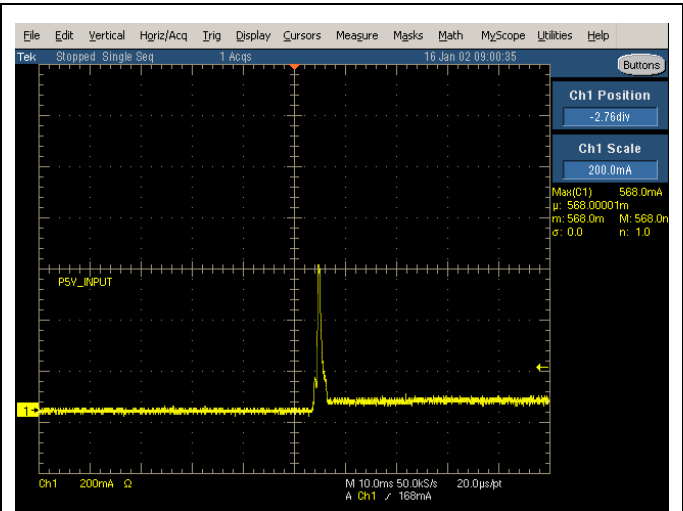
Fig. 4: P5V_INPUT (Zoom in) (AC:110V)
