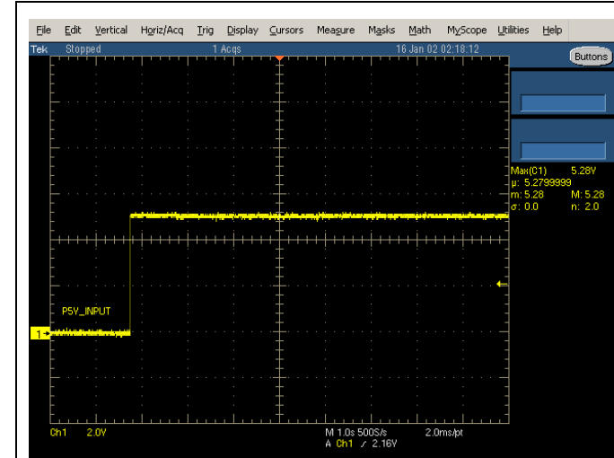
Fig. 1: P5V_INPUT (AC:110V)
